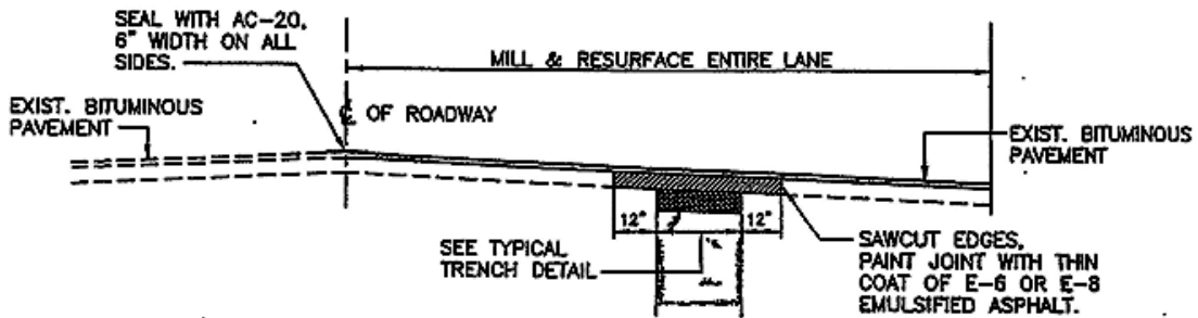
SECTION B-B
